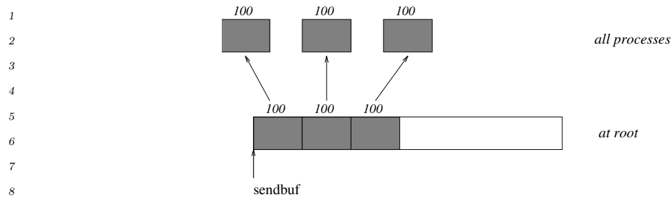
Figure 6.9: The root scatters sets of 100 ints to each MPI process in the group.
