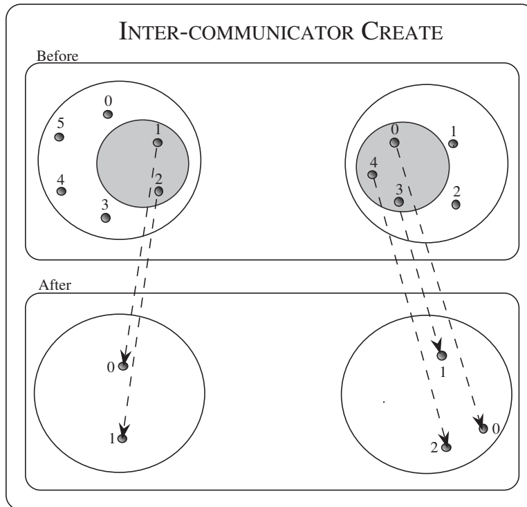
22 Figure 7.1: Inter-communicator creation using MPI_COMM_CREATE extended to inter-communicators. The input groups are those in the grey circle.
