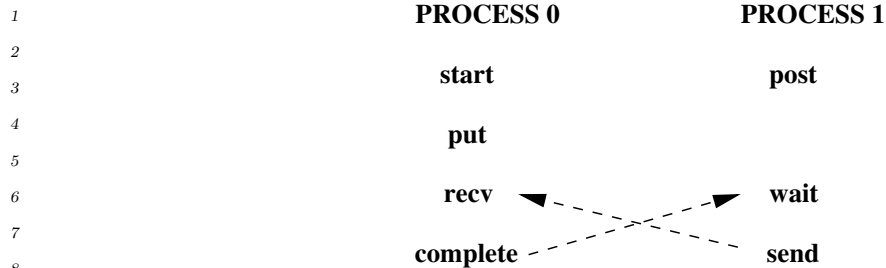
Figure 12.7: Deadlock situation
