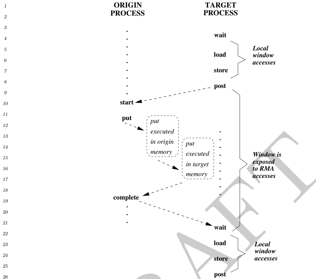
Figure 12.2: Active target communication. Dashed arrows represent synchronizations (ordering of events).
