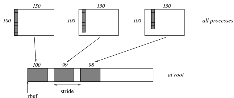
Figure 6.7: The root gathers 100-i ints from column i of a 100 \times 150 C array, and each set is placed stride ints apart.
