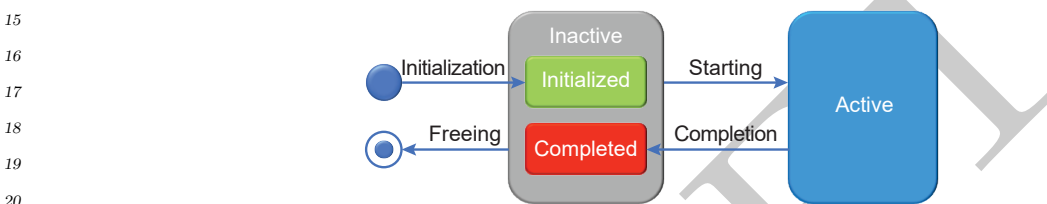
Figure 2.3: State transition diagram for persistent operations
