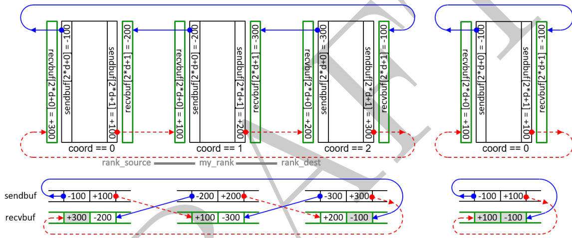
Figure 8.3: Cartesian neighborhood alltoall example for 3 and 1 processes in a dimension.
